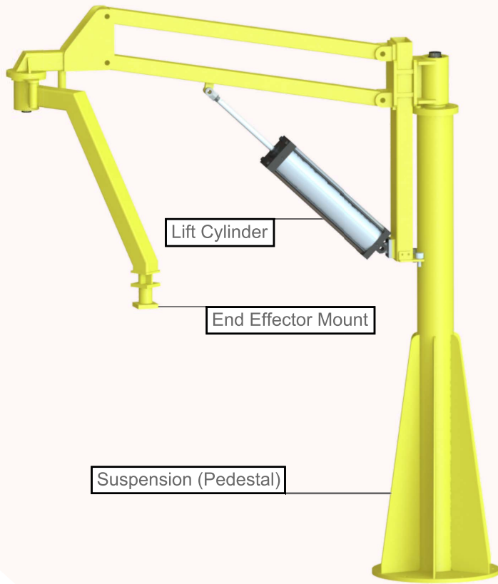
AIMCO Articulating Lifting Arm
